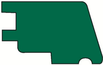
# 197 Sill Nosing 1-3/32 x 1-25/32
