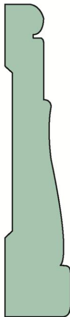
WM 445 C,P,F 11/16 X 3-1/4
