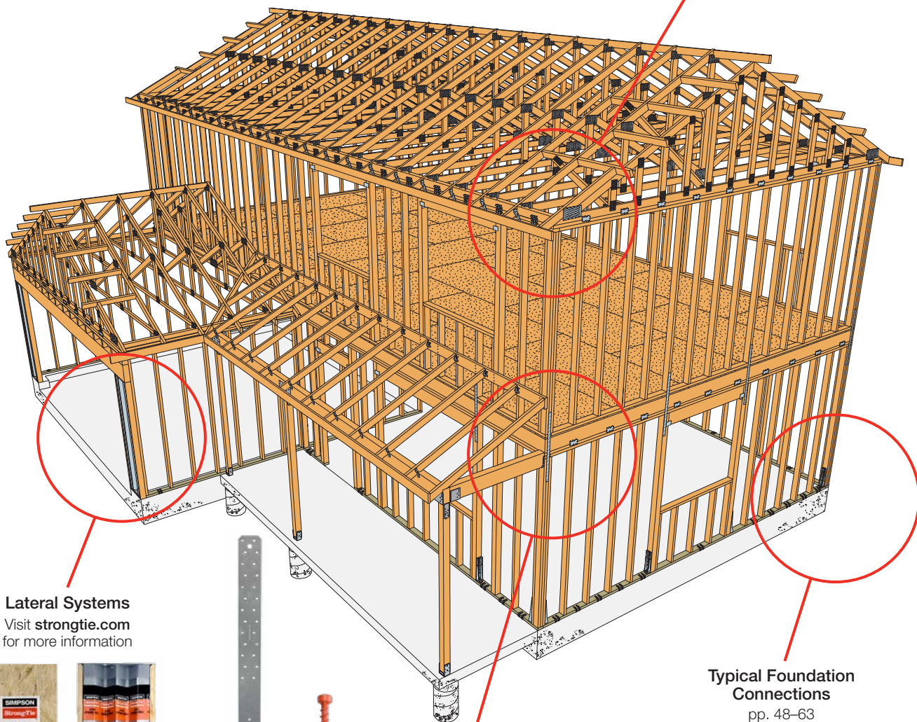
Typical Roof/Wall Connections pp. 314–332
