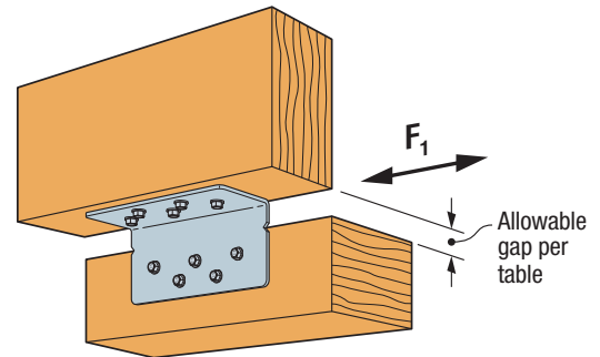
Typical HSLQ37 Installation
