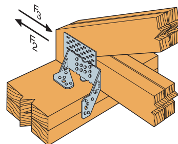
TBE6 Installed on Double 2x8 Top Plate
