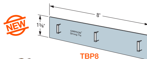
TBP8
