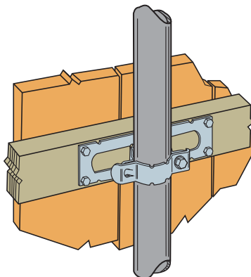
Typical PGT2E Installation
