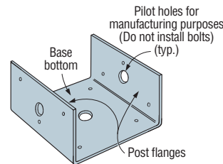
BC60 Half Base (Other similar)
