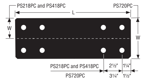
PSPC
