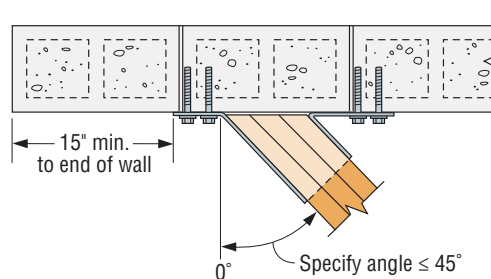
Top View HGUM Skewed Right Bevel Cut
