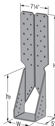
THGQH5.50 (Others similar)
