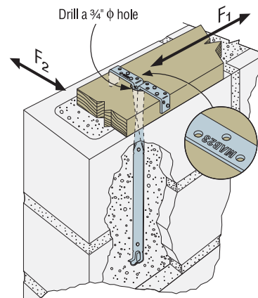
Typical MAB23 Installation in Concrete Block
