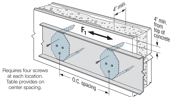
Typical Steel Ledger Installation with ICFVL (Minimum 16 ga. steel ledger)
