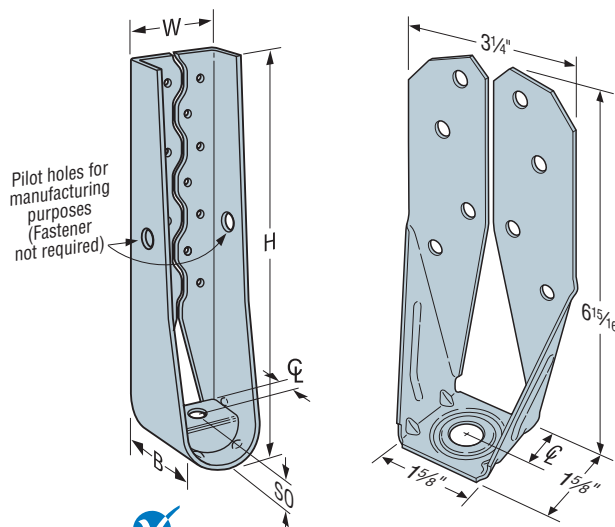
DTT2Z U.S. Patent 8,555,580
