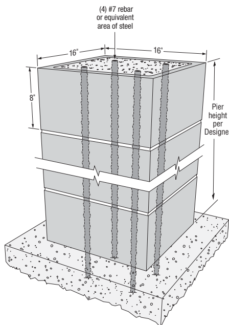
16" Square CMU Pilaster Filled with 3,000 psi Concrete
