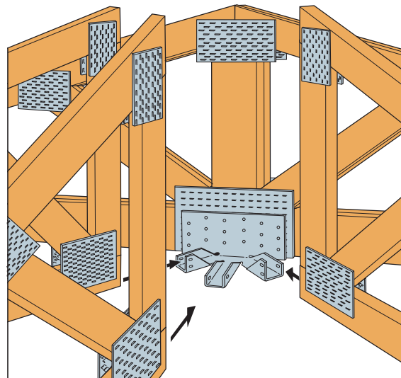
Typical LTHMA Installation
