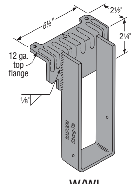
W/WI
