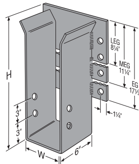
LEG/MEG/EG without Top Flange (See options)
