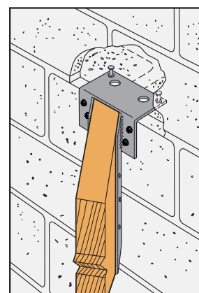
Typical WMU Sloped Down, Skewed Right Block Wall Installation
