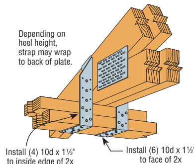
H16-2 Installation
