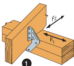
1 H1 Installation
