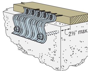
URFP Installed on a Straight Foundation with \frac{1}{2} " Offset Mudsill
