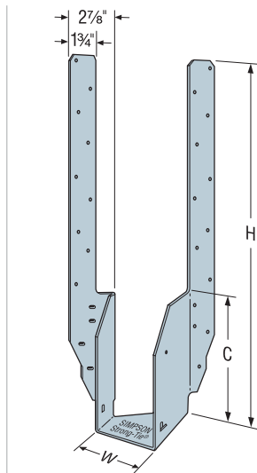
THAR/L422
