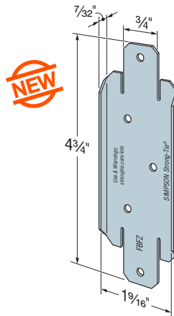
FB24Z
