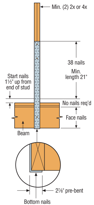
MSTC48B3 Installation with No Rim Board
