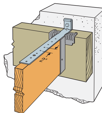
Horizontal LTT19 Installation (LTT20B similar)
