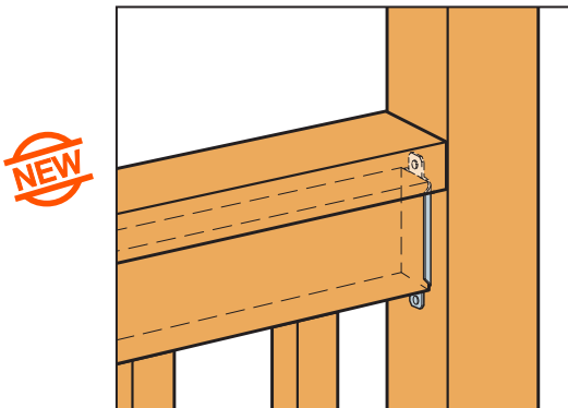
Typical FBFZ Handrail Installation
