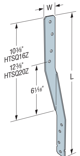
HTSQ16Z (Others similar)
