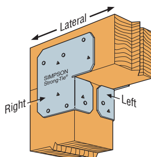
Typical ACE Installation (AC similar)
