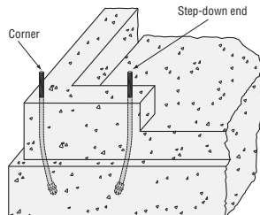
Perspective View
