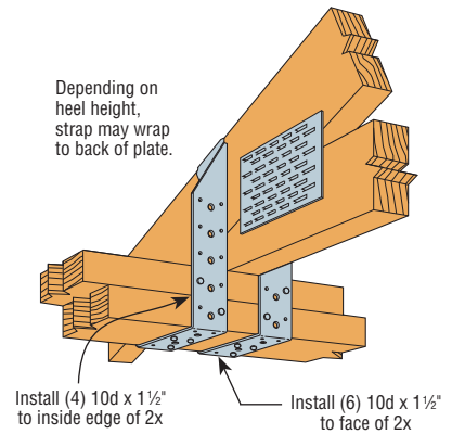
H16 Installation
