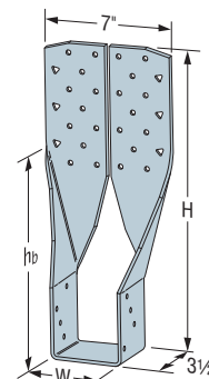
THGQ3.62 (Others similar)
