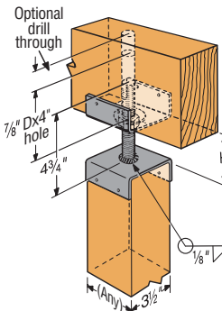
Two Methods of JP44 Installation
