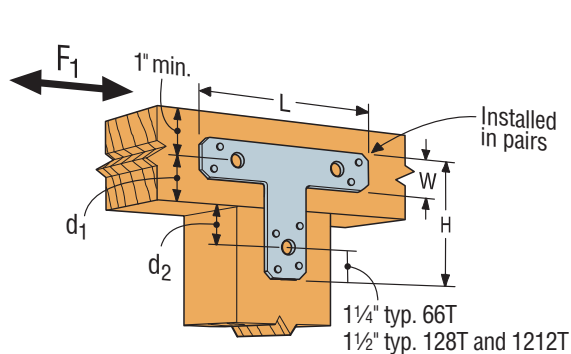
Typical T Installation
