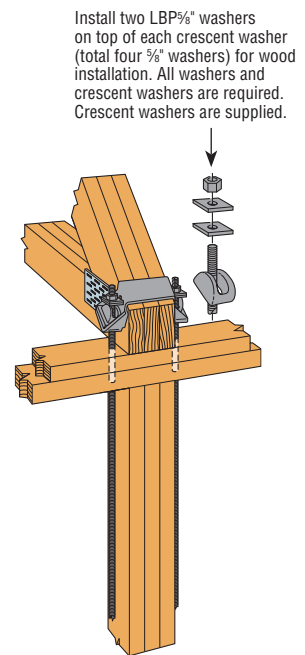
Typical HGT-3 Installation with Full-Height Threaded Rod
