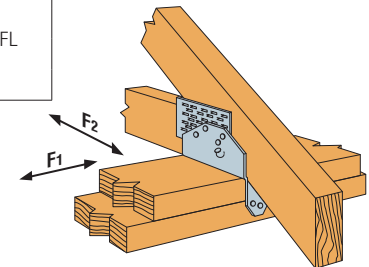
HS24 U.S. Patents 5,603,580
