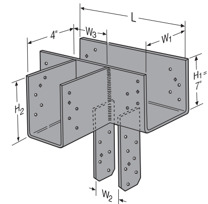
CCTQ-SDS2.5
