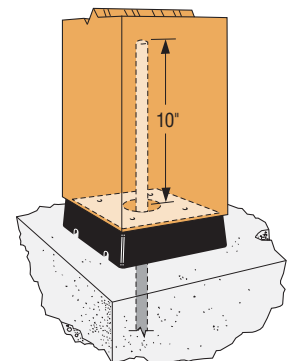
Typical CPS4 Installation
