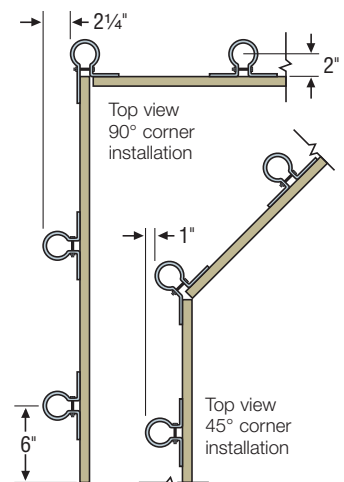
Corner Installation Top View
