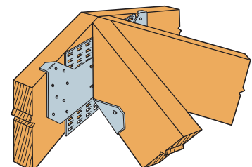
Optional Installation for HRC22 Only
