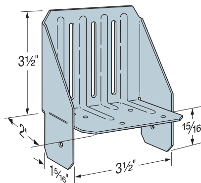
HTC4
