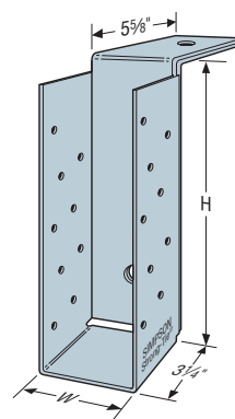
MBHA
