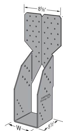
THGQH3-SDS4.5 (THGQH4-SDS6 similar)
