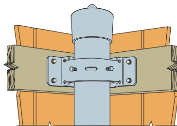
Typical PGTIC2Z-R Fence Installation
