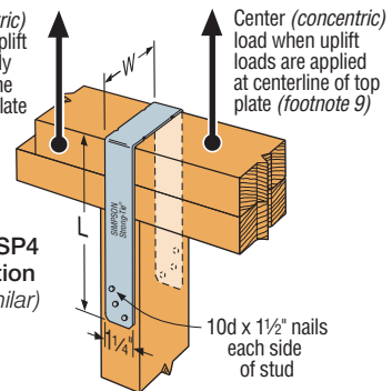
Typical TSP Installed to Top Plate
