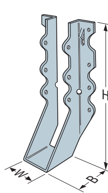
LU28 (Except LU roughs)
