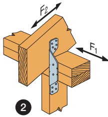
2 H2A Installation
