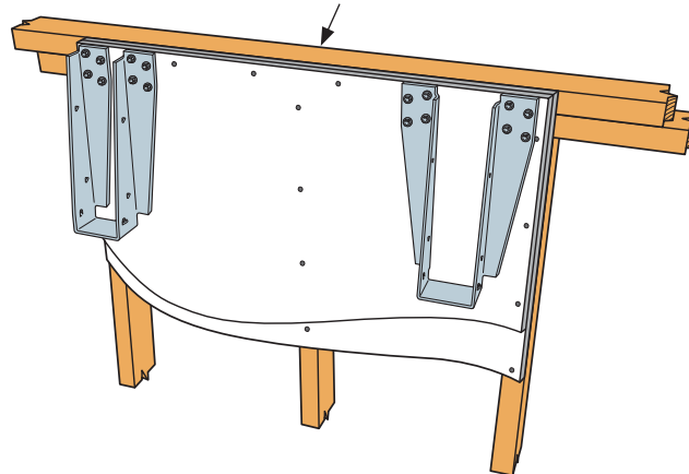
Typical Installation Showing DHU with Concealed Flange Option (at left) and a DHU Standard Installation
