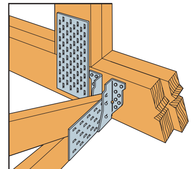
Typical HUS26 Installation with Reduced Heel Height
