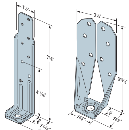
DTT1Z U.S. Patent Pending
