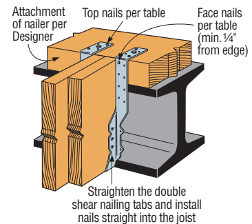
Typical THA Top Flange Installation on a Nailor (except THA29)
