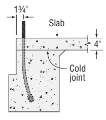
Two-Pour Installation
