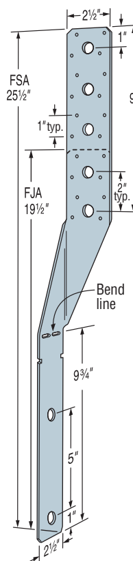
FJA/FSA
