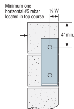
Installation on End of Wall (Minimum load)
