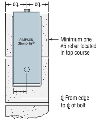
Typical MBHA Installation
