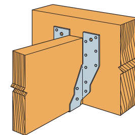
Typical THA29 Face-Mount Installation
