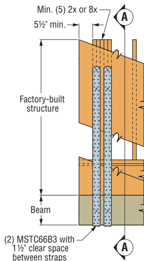
(2) MSTC66B3 Installation
