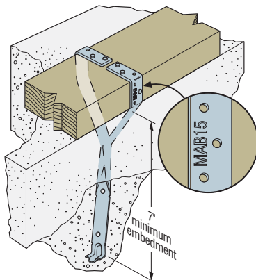
Typical MAB15 Installation in Concrete
