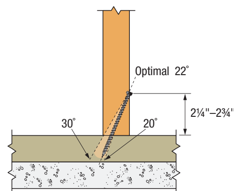
Stud-to-Bottom Plate Connection Over Concrete/Masonry Foundation (This application requires Strong-Drive SDWC15450)
