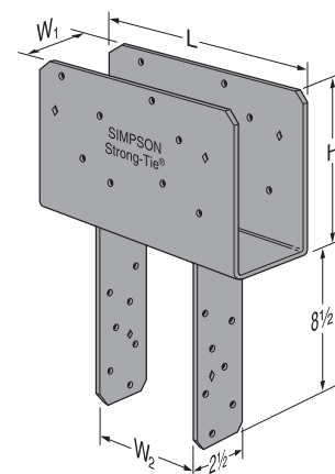
CCQ46SDS2.5
