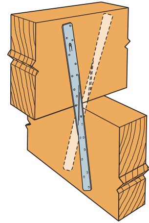
Typical TS Installation
