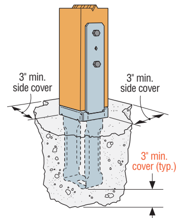
Typical CBS Installation
