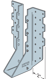
✓ HUS210 (HUS26, HUS28, and HHUS similar)
