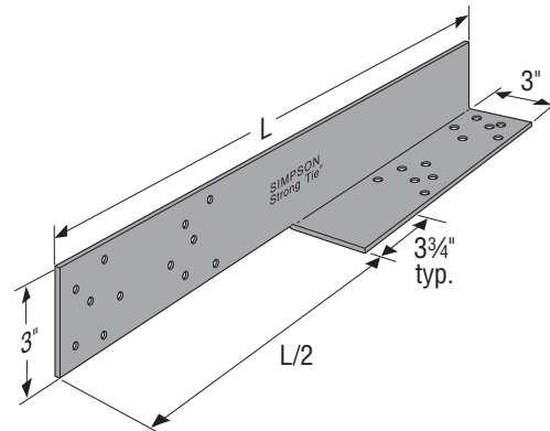
DSC5R/L-SDS3
