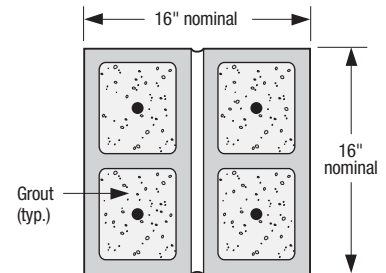
16" Square Grout-Filled CMU (Plan view)
