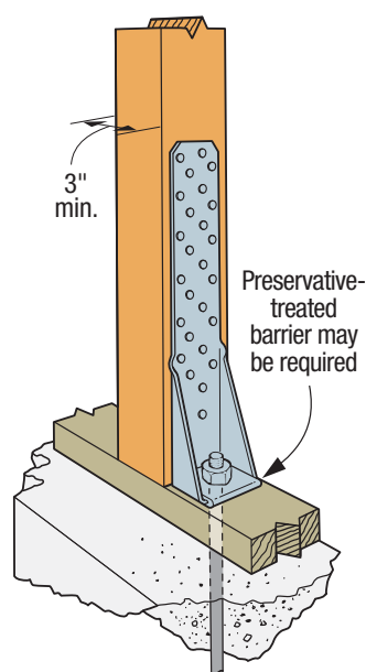
Vertical HTT4 Installation See p. 306 for marriage strap at panelized roof applications.
