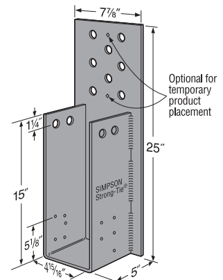
THGBH3 (THGBH2 and THGBH4 similar)
