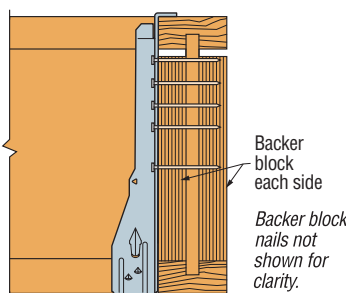
Face-Mount Hanger
