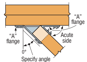
Top View HTU Hanger Skewed Right < 51°
