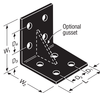
HL55PC
