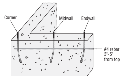
Perspective View
