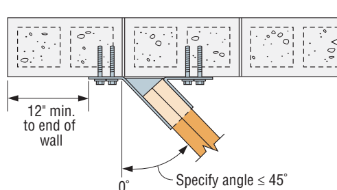
Top View LGUM Skewed Right Square Cut
