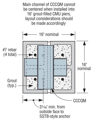
CCCQM Installed on 16" Square Grout-Filled CMU (Plan view)
