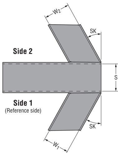
GLS (Skewed Inward) Skewed Left, Offset Left (Top View)
