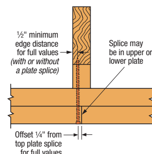
Min. Edge Distance for Top Plate Splice
