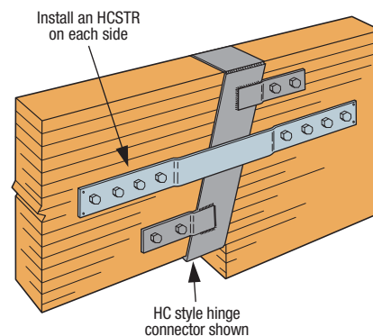
Typical HCSTR4 Installation
