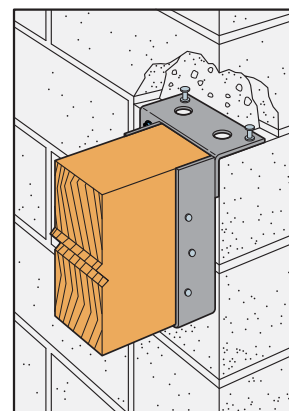
Typical WMU Top Flange Offset Left
