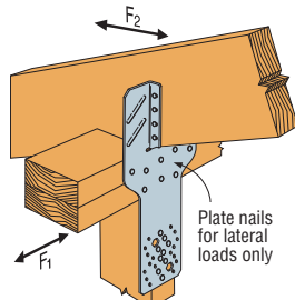
15 H10S Installation
