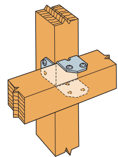
RTB22 Installation
