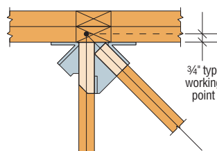
Top View Right-Hand Hip Installation
